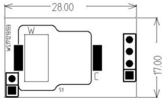
Fig1. Structure
